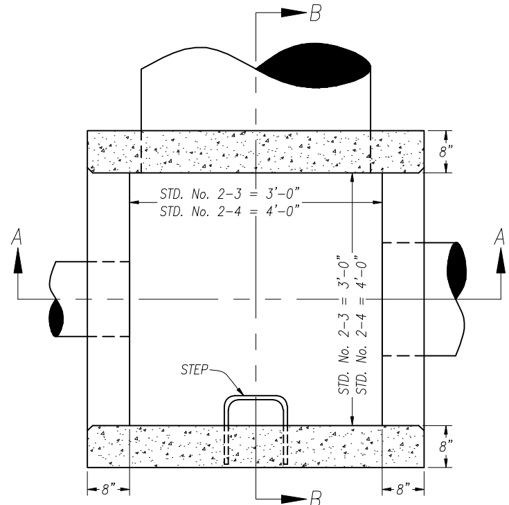
SECTION C-C
