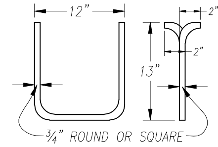
STEP DETAIL
