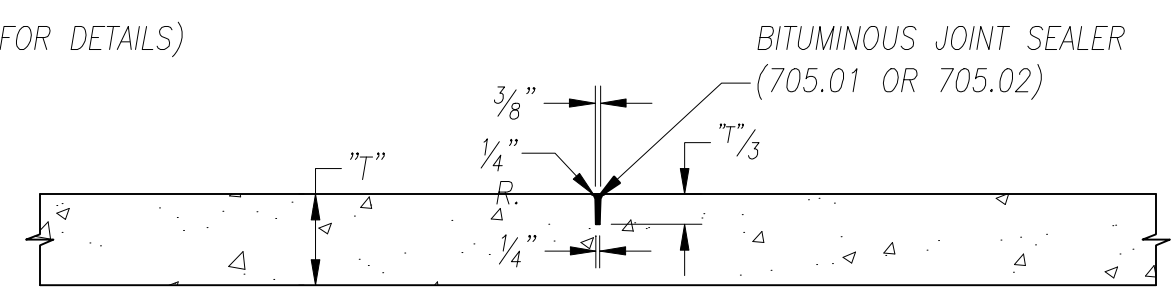
CONTRACTION JOINT (SPACED AT THE DIRECTION OF THE ENGINEER)
